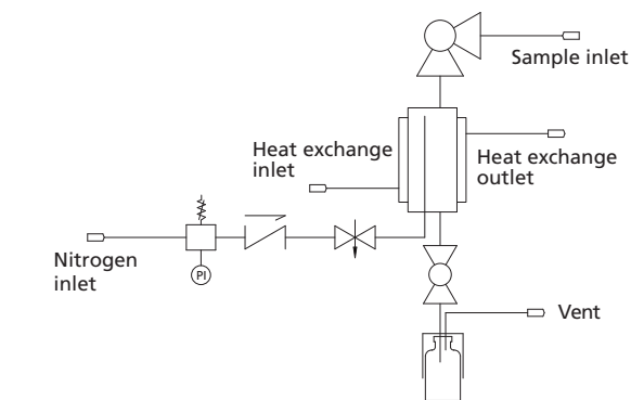
Schematic diagram
