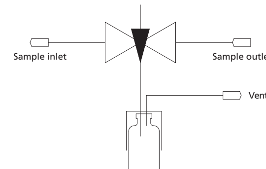
Schematic diagram
