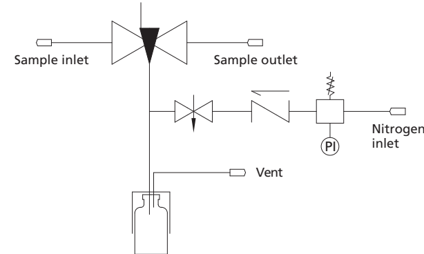
Schematic diagram
