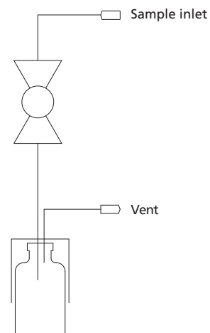
Schematic diagram
