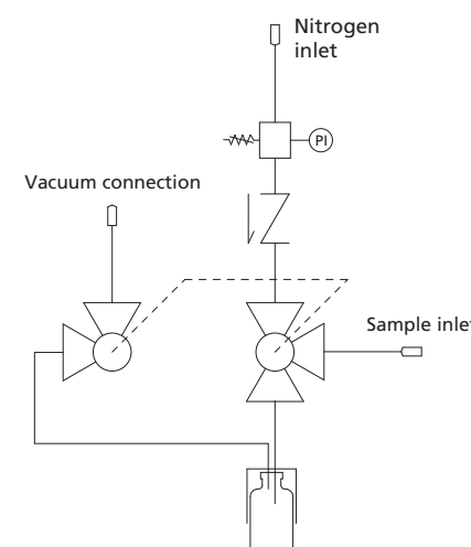
Schematic diagram
