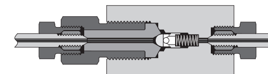
60CO Series (Ball Check Valves)
