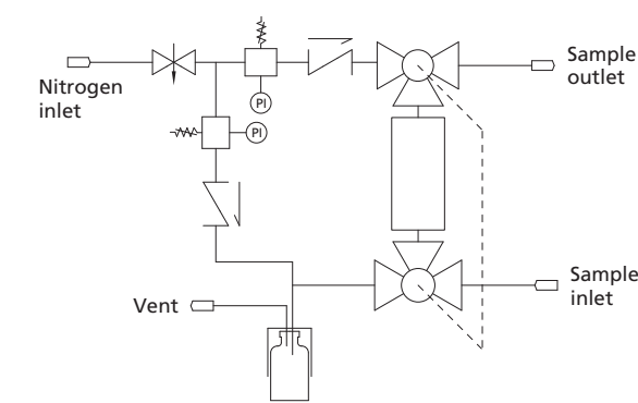
Schematic diagram
