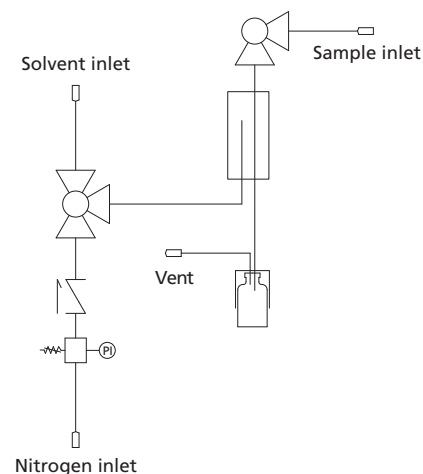
Schematic diagram
