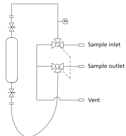
Schematic diagram
