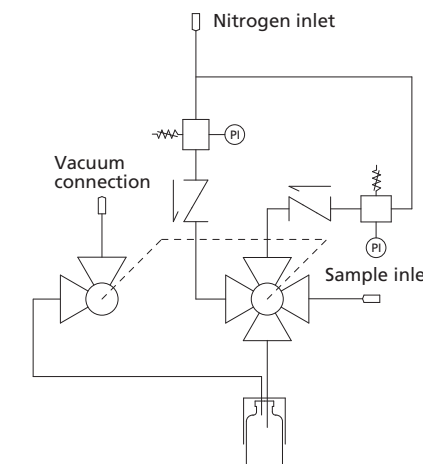
Schematic diagram
