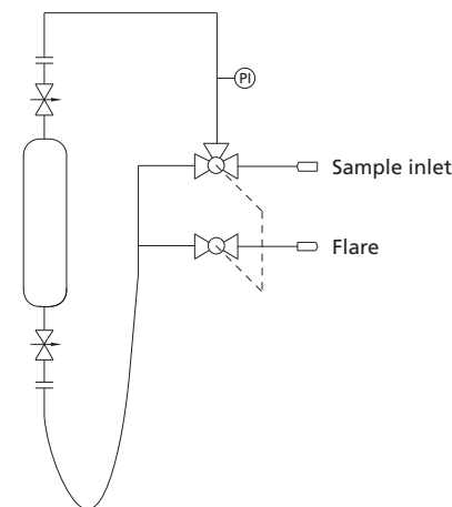
Schematic diagram
