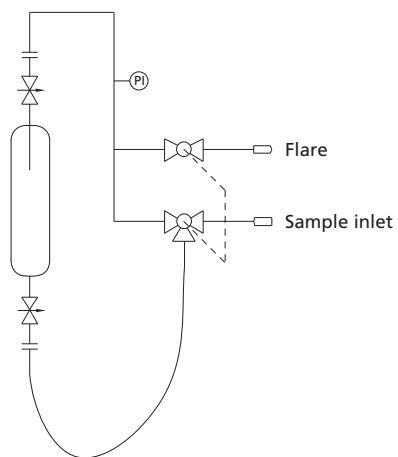
Schematic diagram
