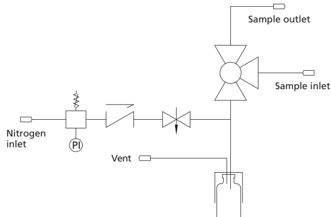
Schematic diagram
