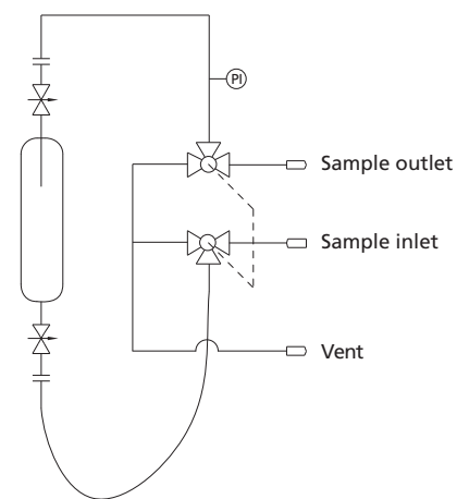
Schematic diagram
