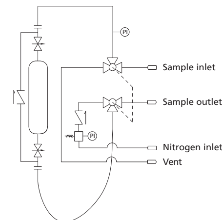
Schematic diagram
