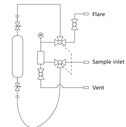
Schematic diagram
