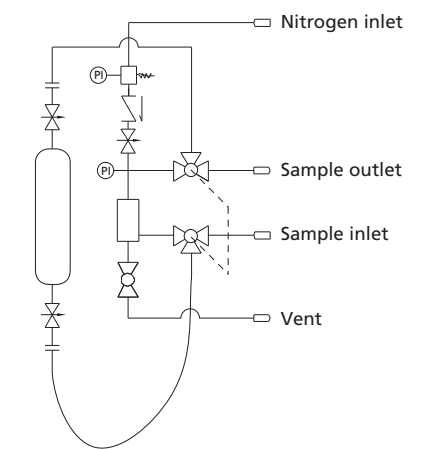
Schematic diagram
